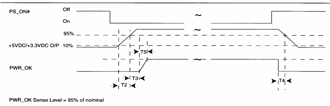
Figure 1: Power Supply Timing
